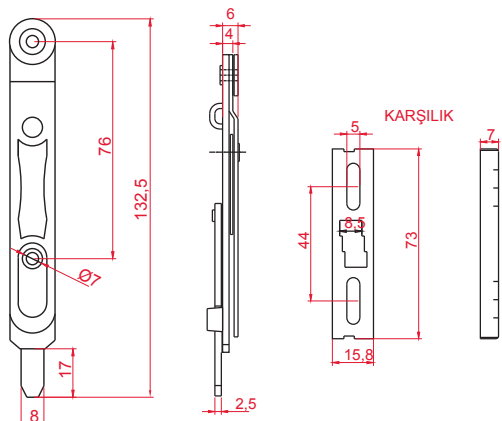
BİNİLİ KAPI SÜRGÜ | SAC DOUBLE SASH SLIDING SHOOT BOLT | STEEL
